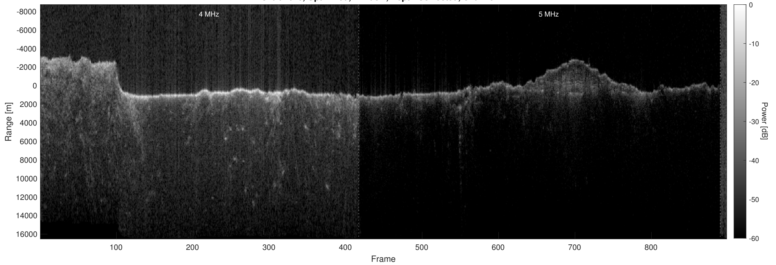
Orbit 4646, Optimized, Window, Depth-Corrected, Channel 2
