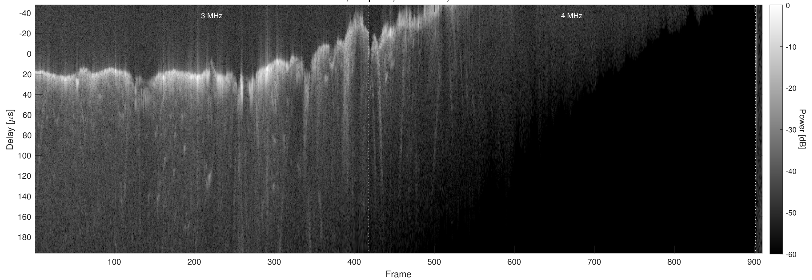
Orbit 4647, Chapman, No Window, Channel 2
