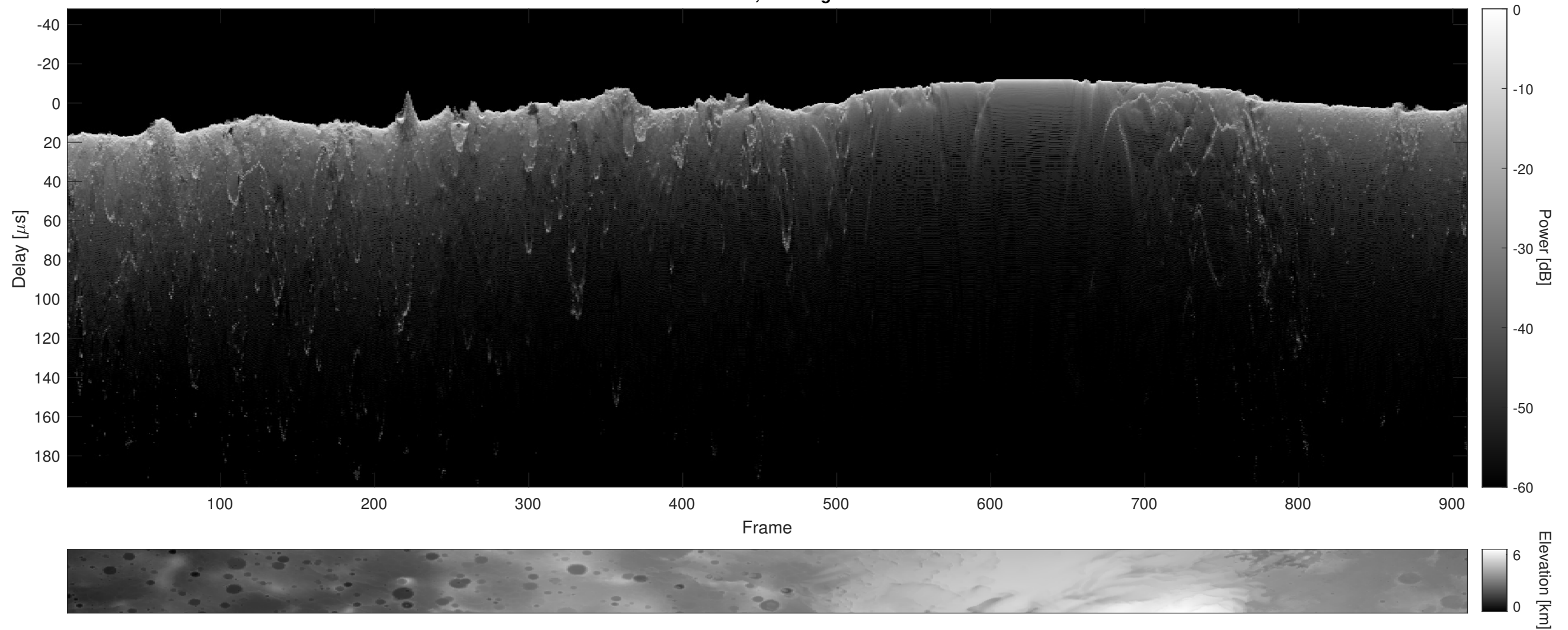
Orbit 4647, Cluttergram
