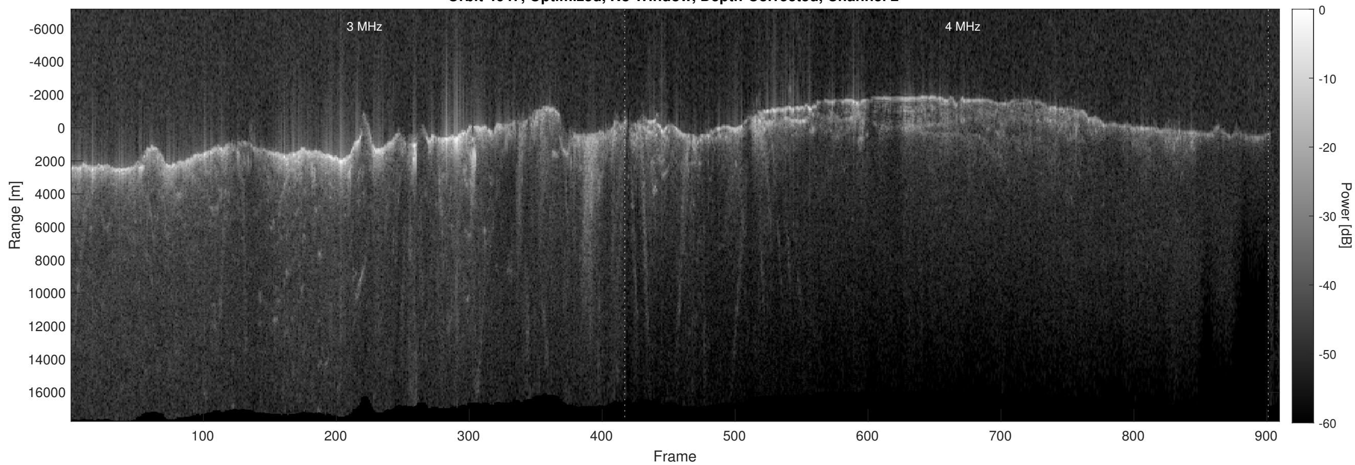
Orbit 4647, Optimized, No Window, Depth-Corrected, Channel 2
