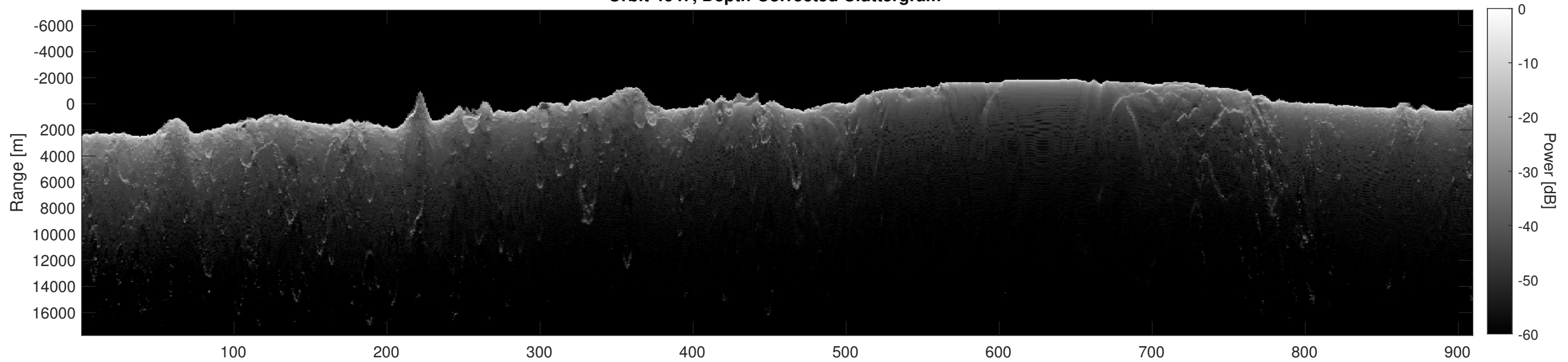
Orbit 4647, Depth-Corrected Cluttergram
