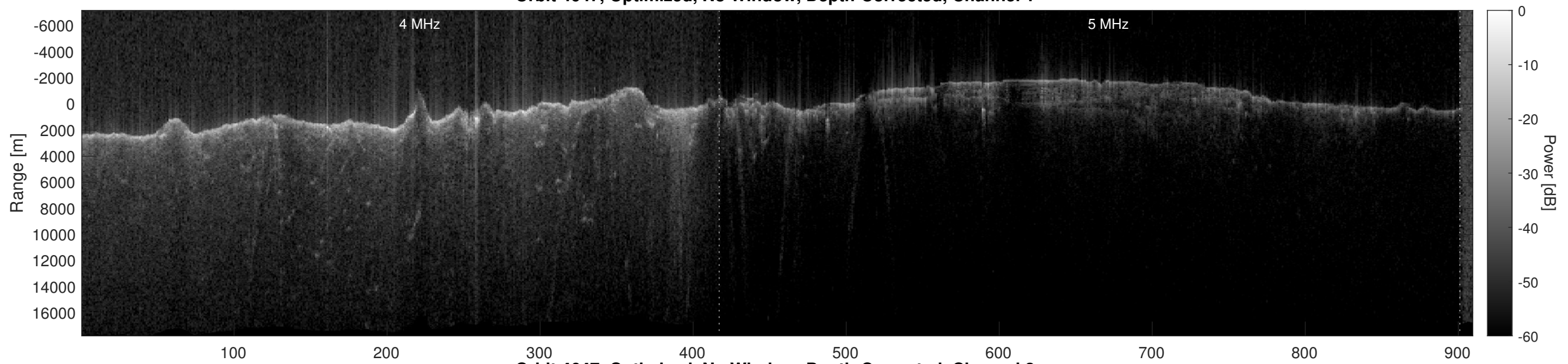
Orbit 4647, Optimized, No Window, Depth-Corrected, Channel 2
