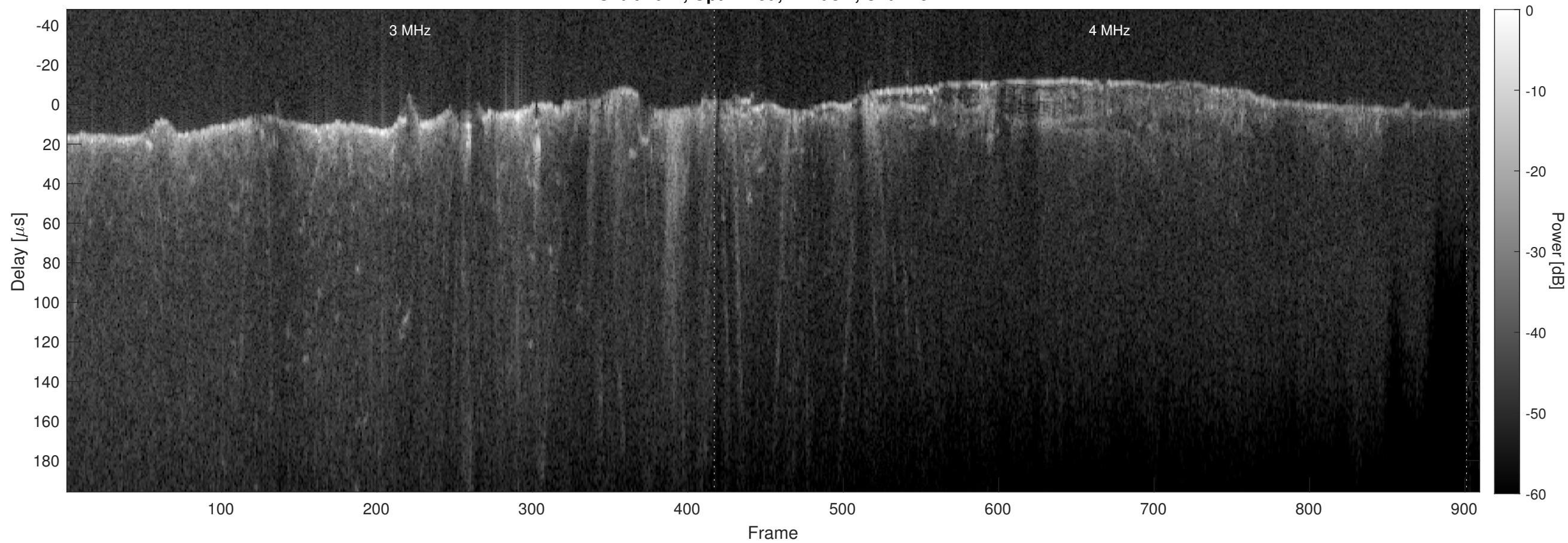
Orbit 4647, Optimized, Window, Channel 2
