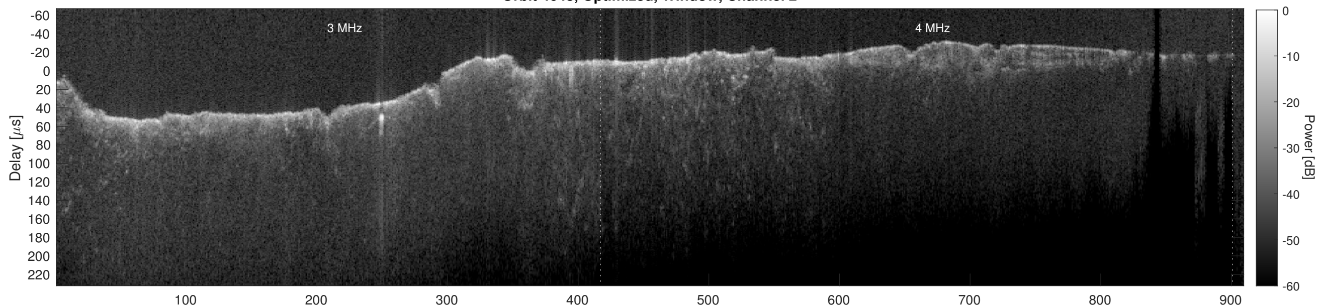
Orbit 4648, Cluttergram
