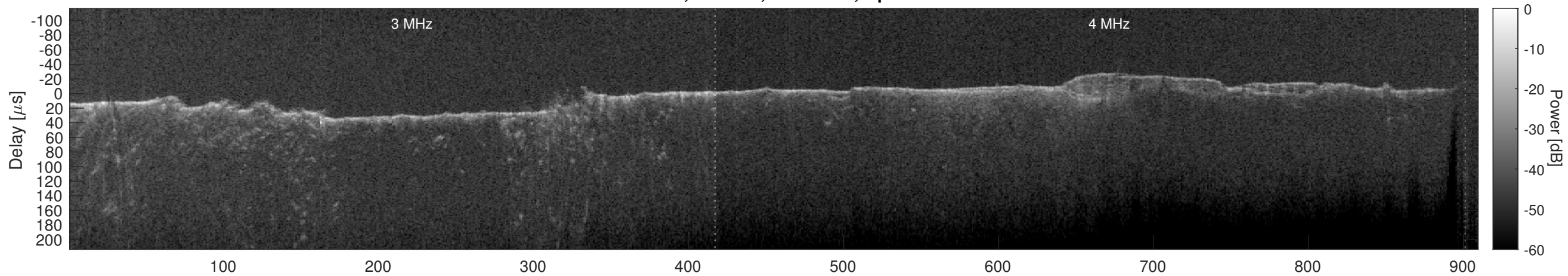
Orbit 4649, Cluttergram
