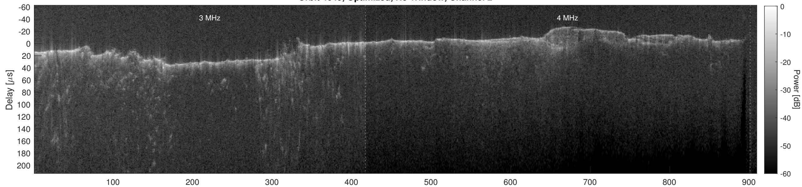
Orbit 4649, Cluttergram
