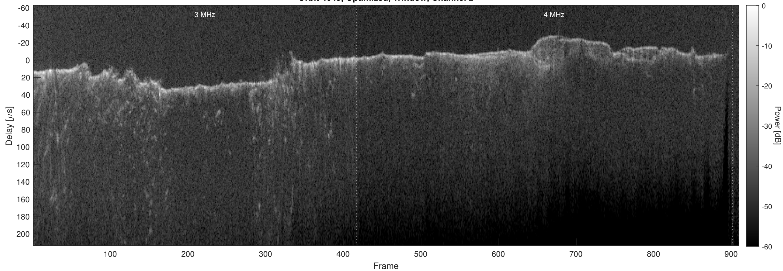
Orbit 4649, Optimized, Window, Channel 2
