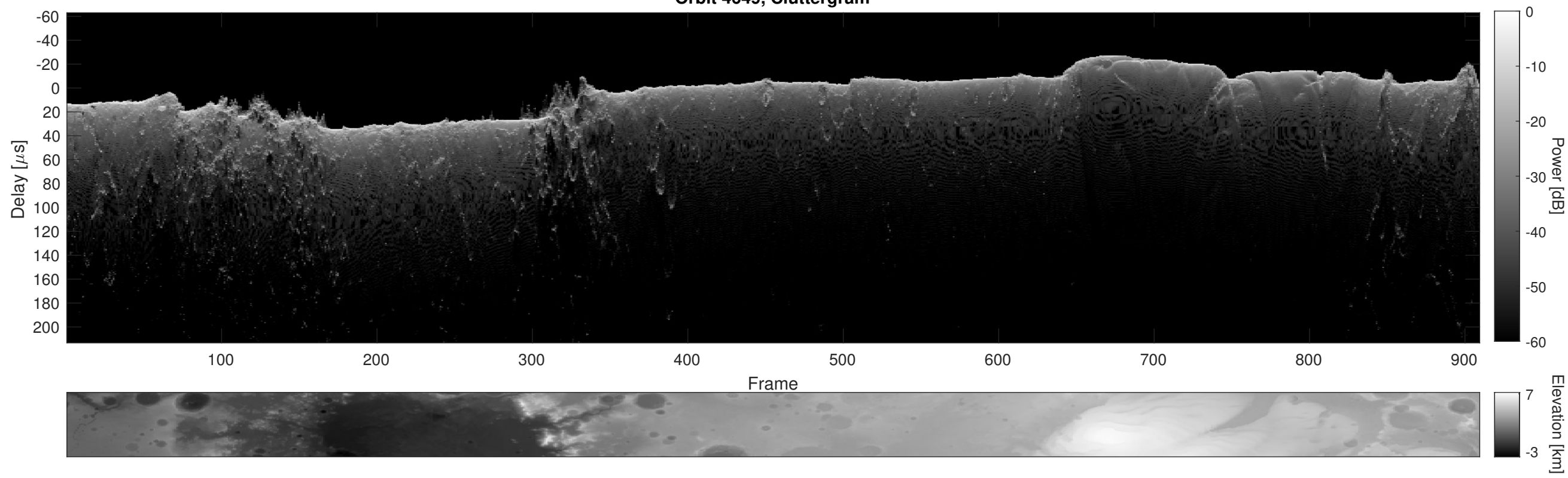
Orbit 4649, Cluttergram
