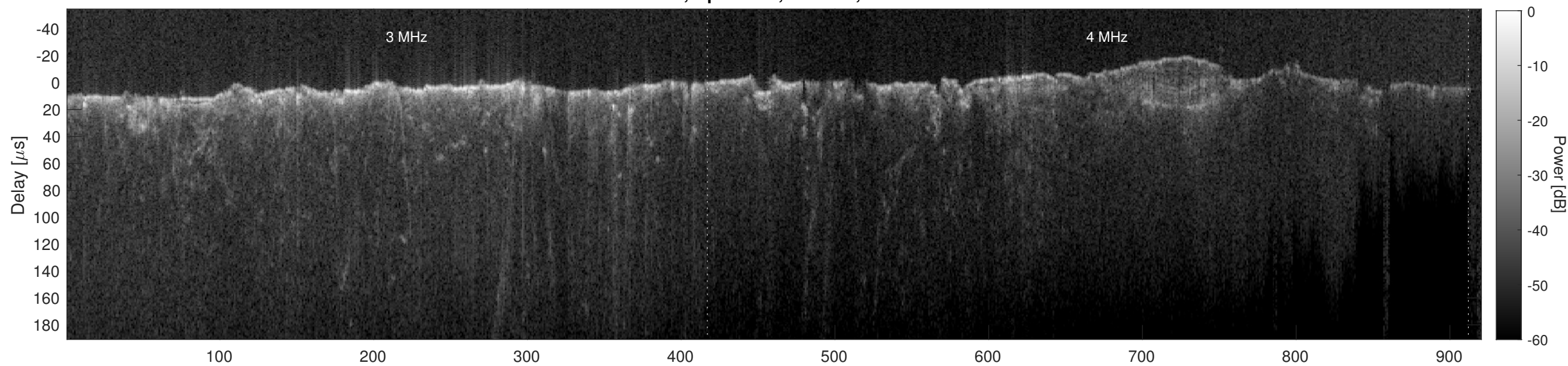
Orbit 4650, Cluttergram
