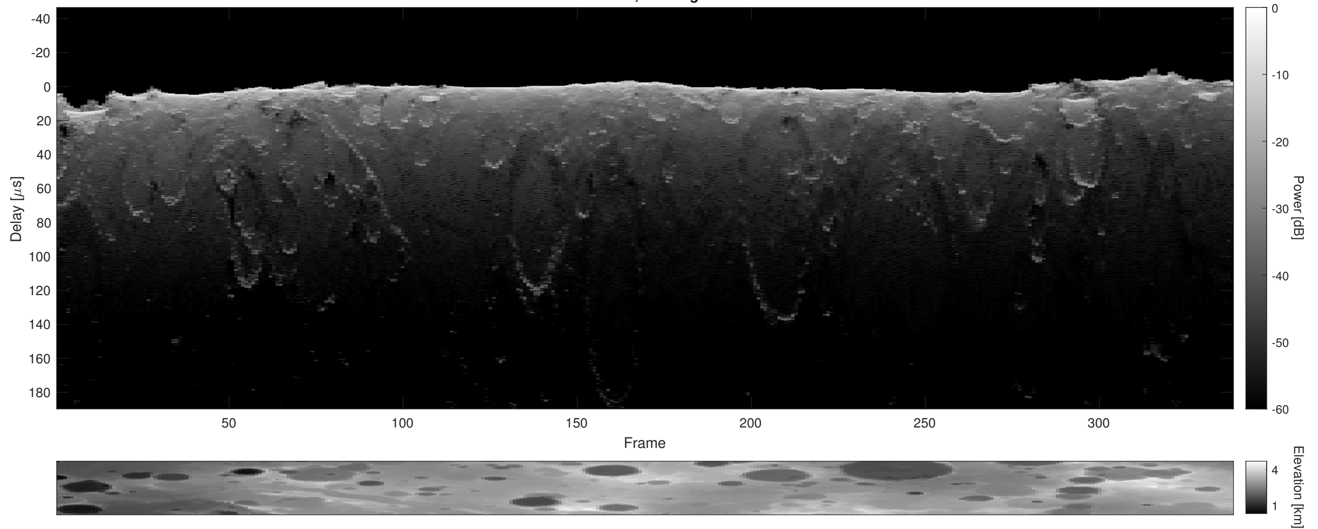
Orbit 4652, Cluttergram
