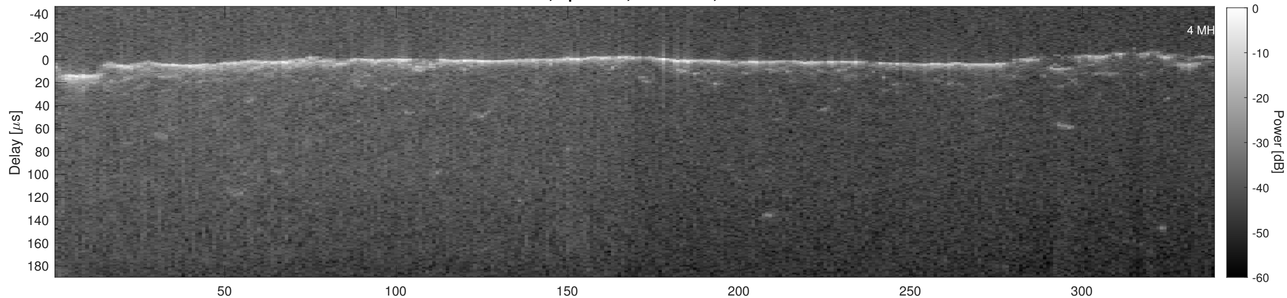
Orbit 4652, Cluttergram
