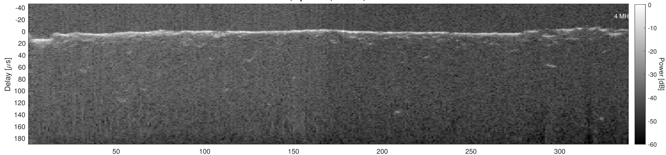
Orbit 4652, Cluttergram
