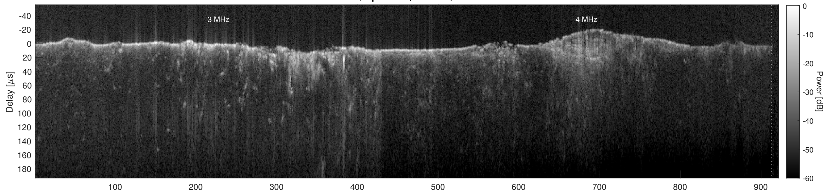
Orbit 4653, Cluttergram
