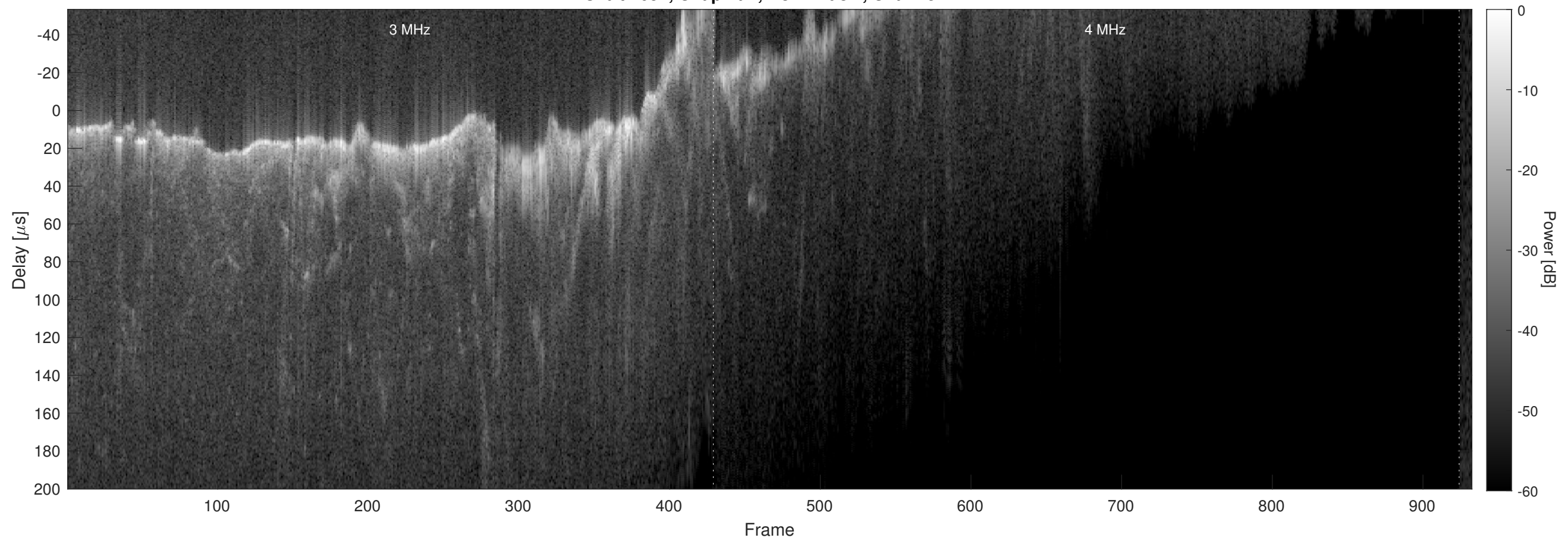
Orbit 4654, Chapman, No Window, Channel 2
