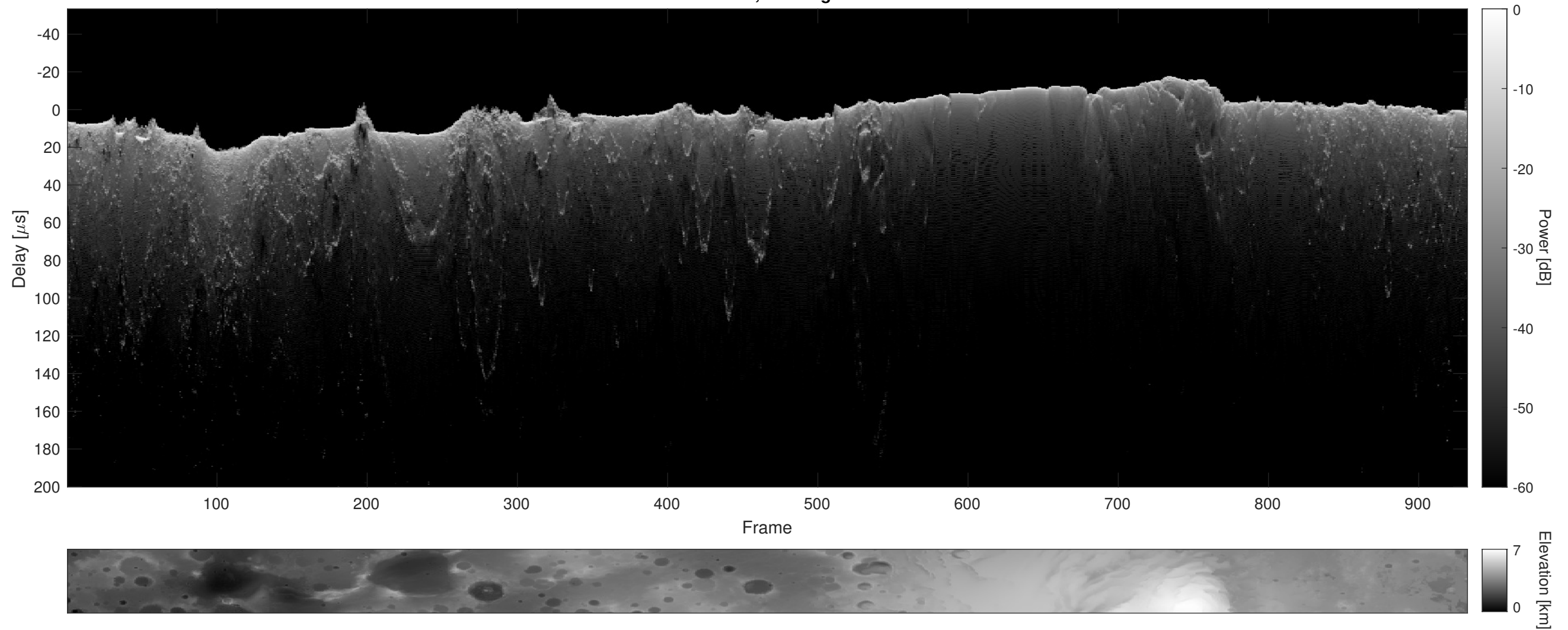
Orbit 4654, Cluttergram
