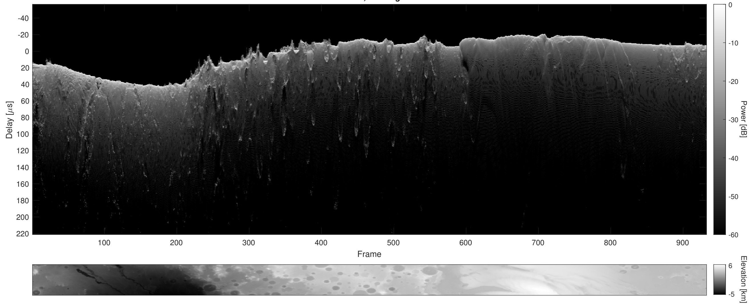
Orbit 4655, Cluttergram
