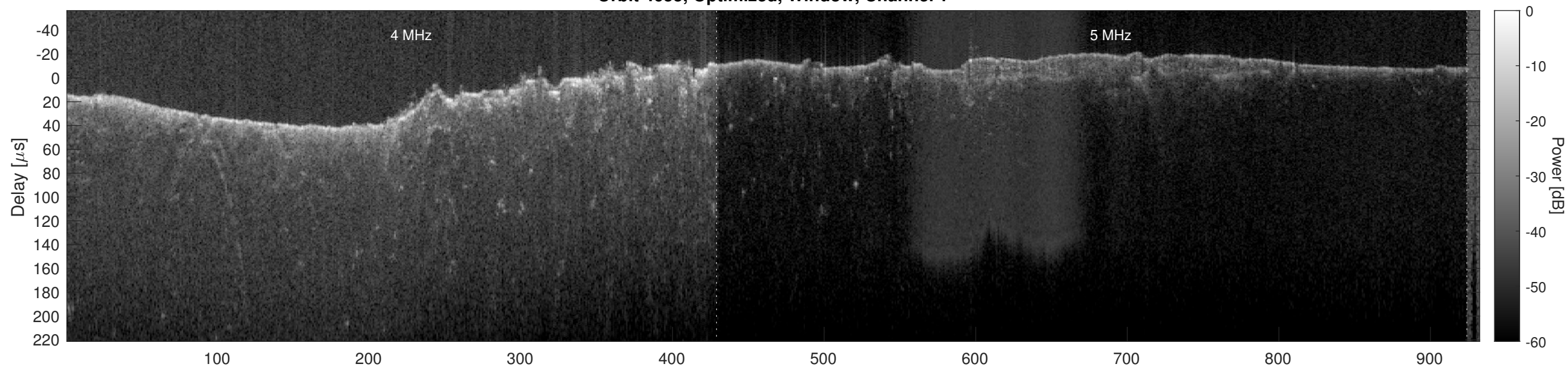
Orbit 4655, Optimized, Window, Channel 2
