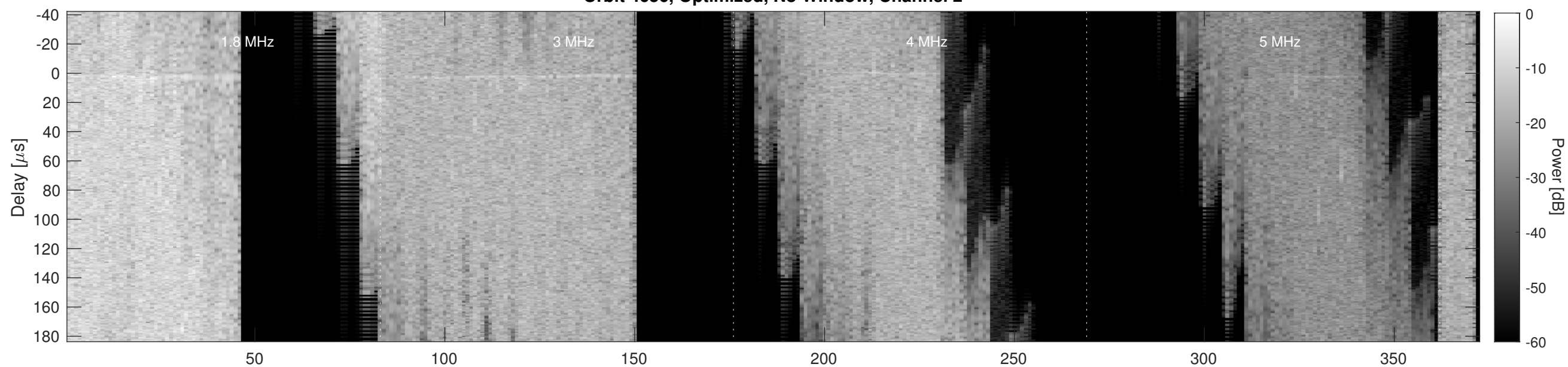
Orbit 4656, Cluttergram
