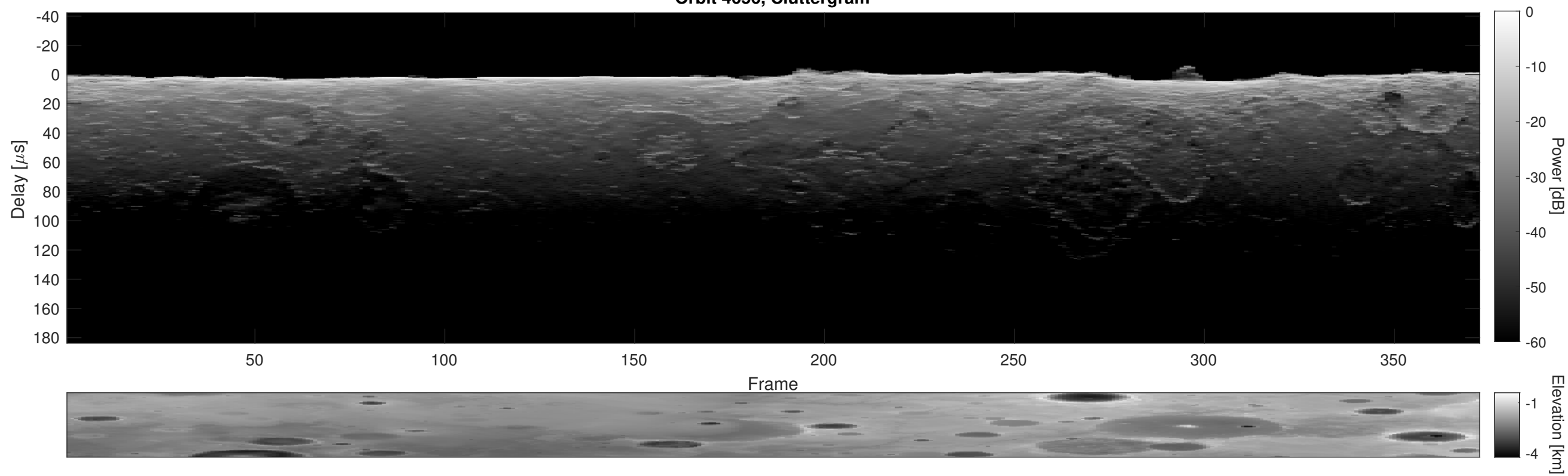
Orbit 4656, Cluttergram
