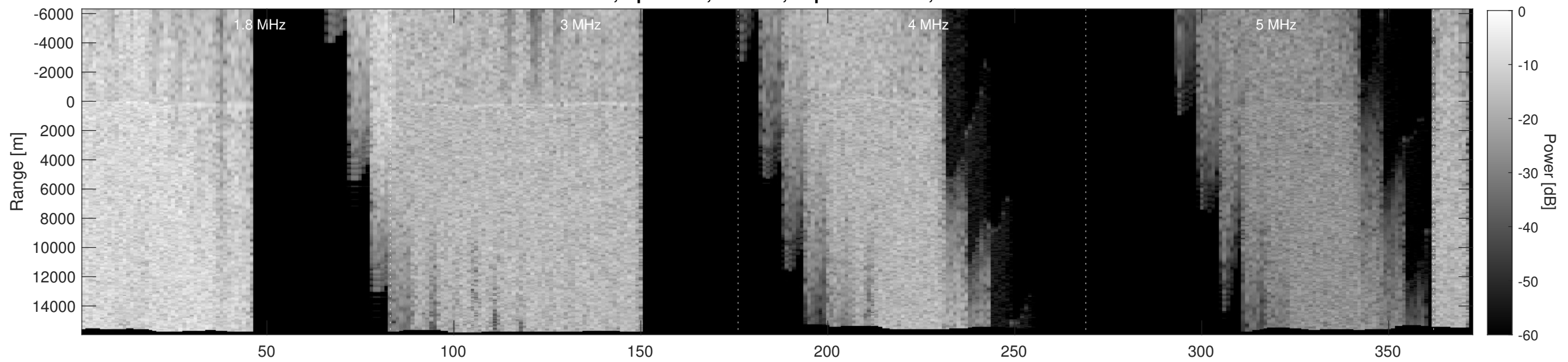
Orbit 4656, Depth-Corrected Cluttergram
