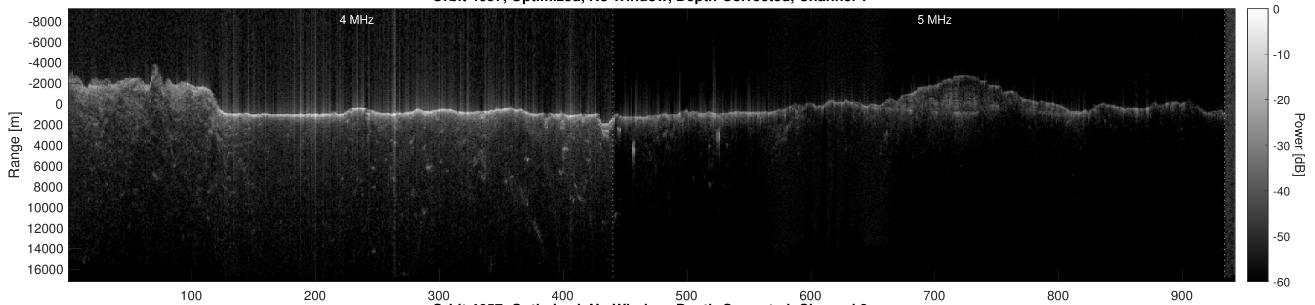
Orbit 4657, Optimized, No Window, Depth-Corrected, Channel 2
