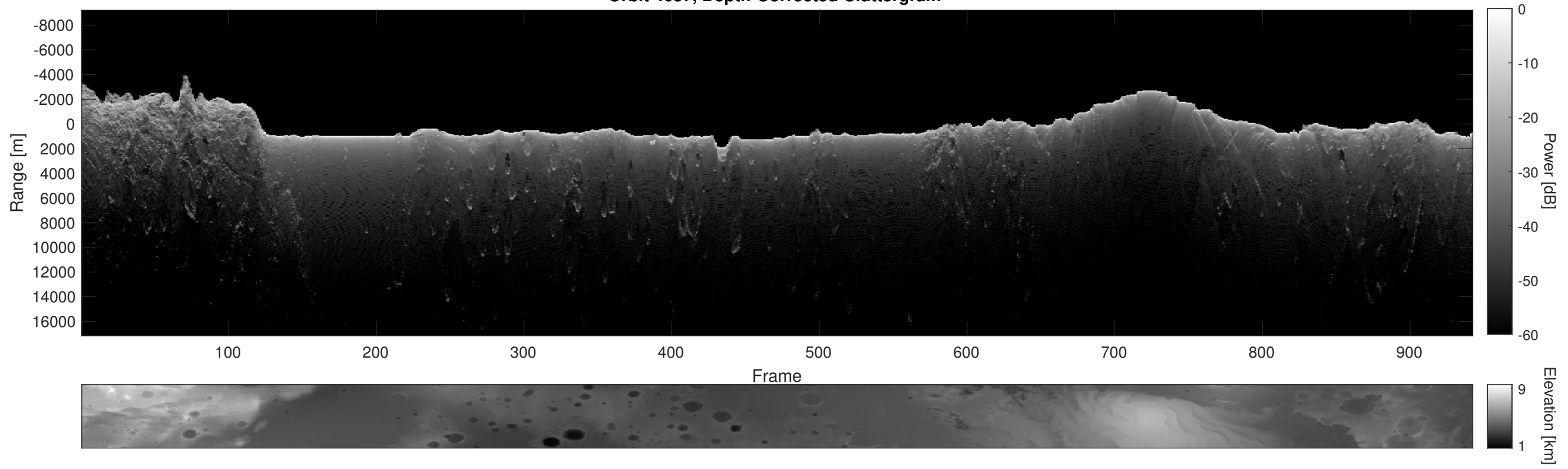
Orbit 4657, Depth-Corrected Cluttergram
