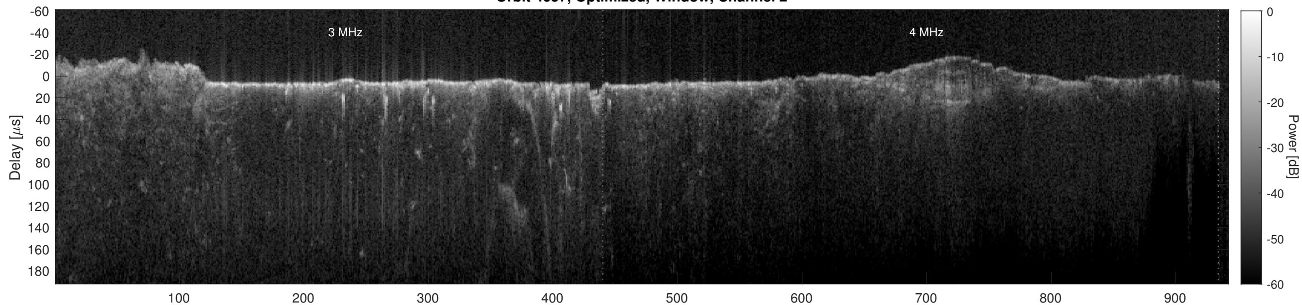
Orbit 4657, Cluttergram
