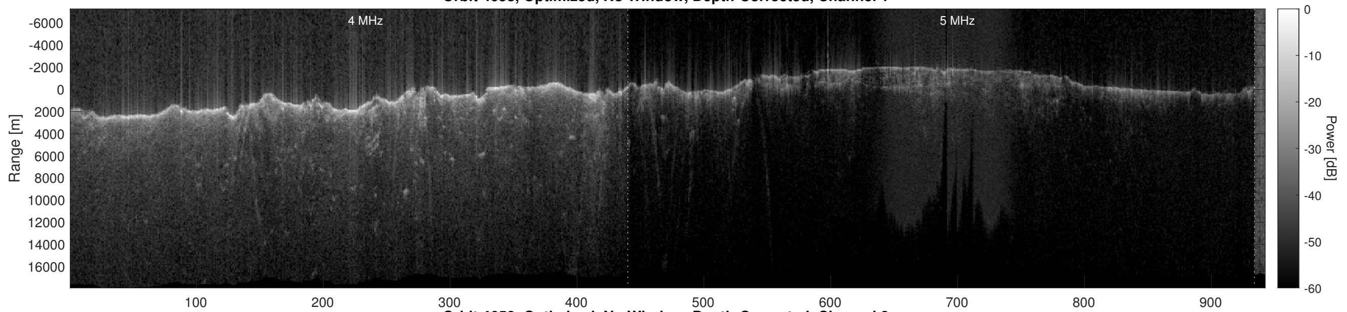
Orbit 4658, Optimized, No Window, Depth-Corrected, Channel 2
