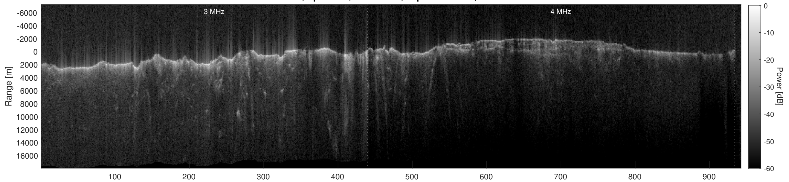
Orbit 4658, Depth-Corrected Cluttergram
