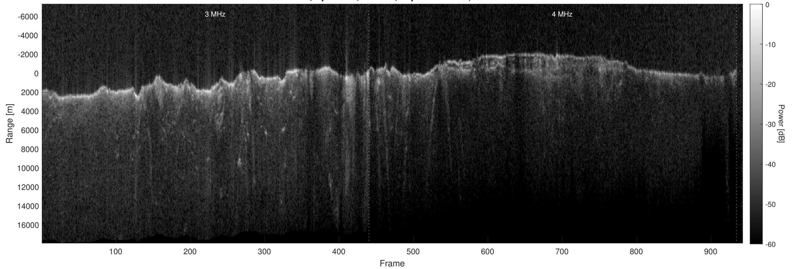
Orbit 4658, Optimized, Window, Depth-Corrected, Channel 2
