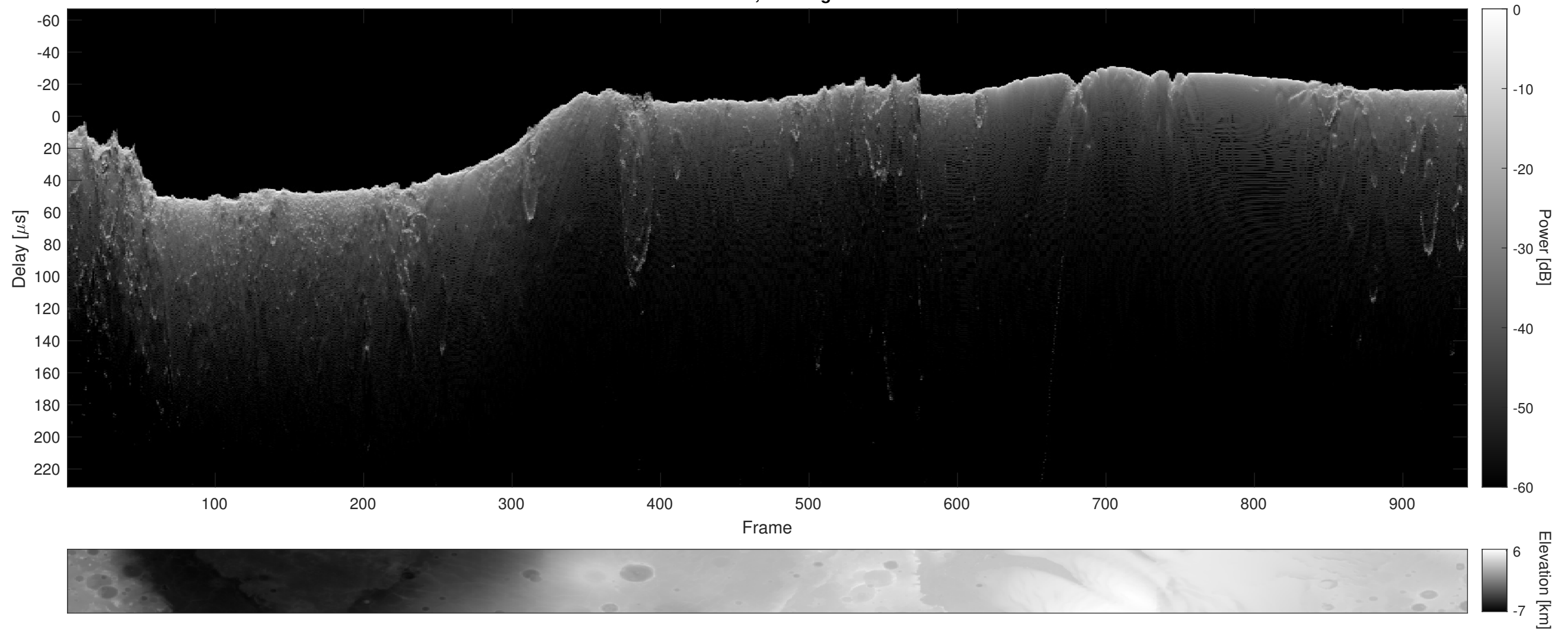
Orbit 4659, Cluttergram
