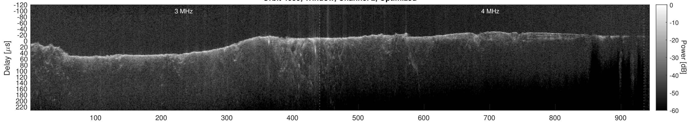
Orbit 4659, Cluttergram
