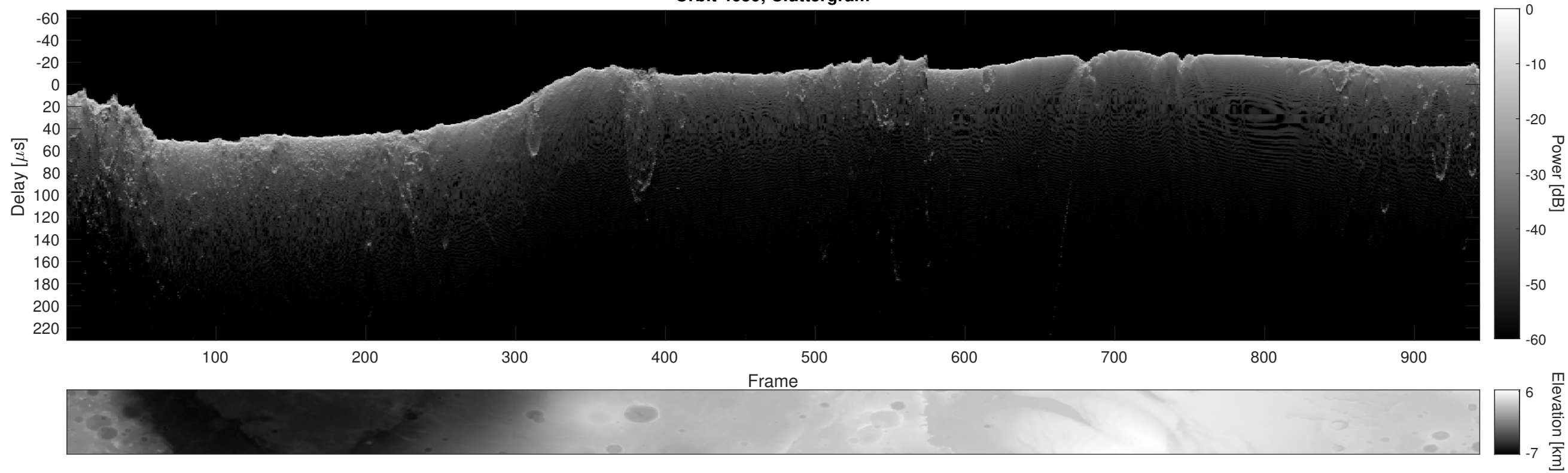
Orbit 4659, Cluttergram
