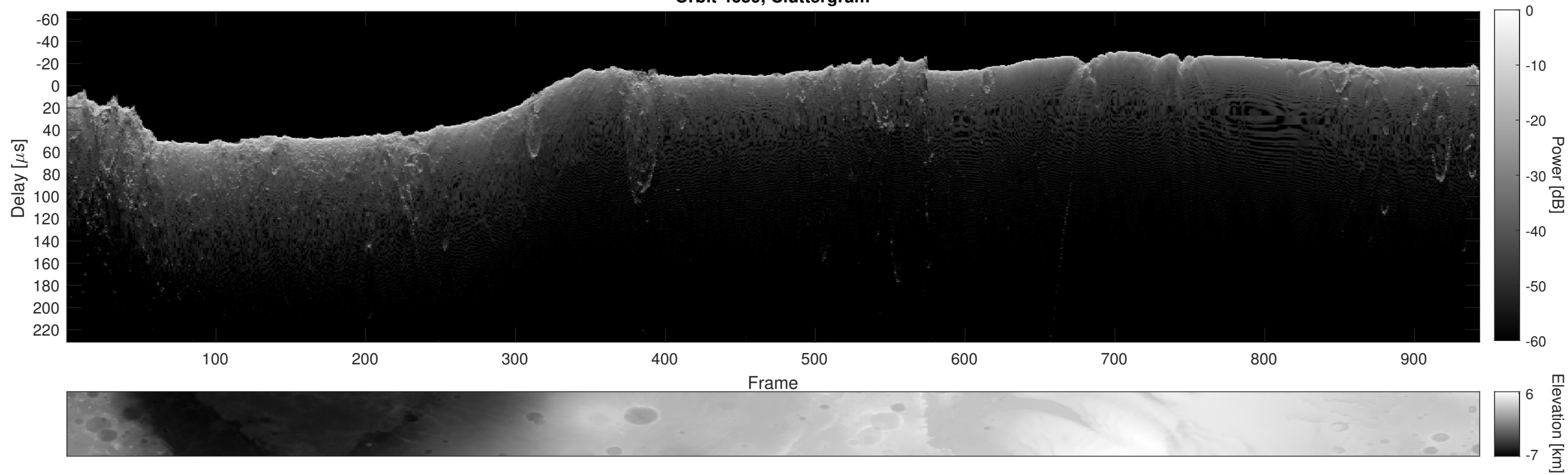
Orbit 4659, Cluttergram
