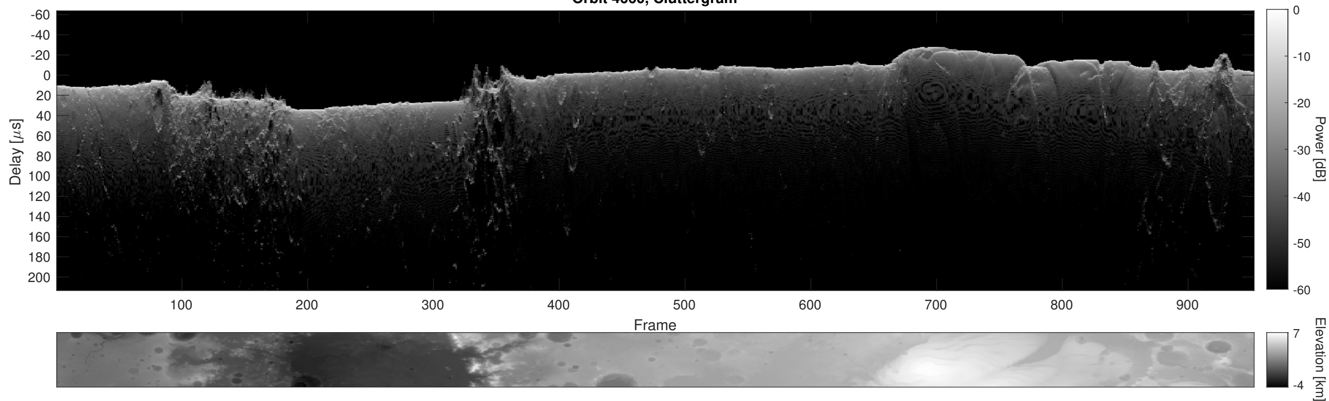
Orbit 4660, Cluttergram
