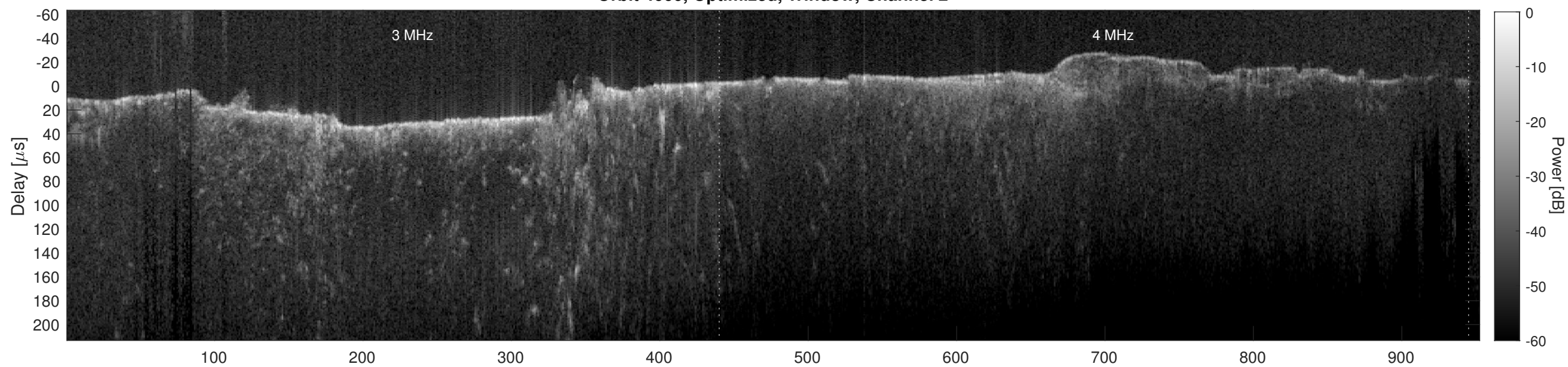
Orbit 4660, Cluttergram
