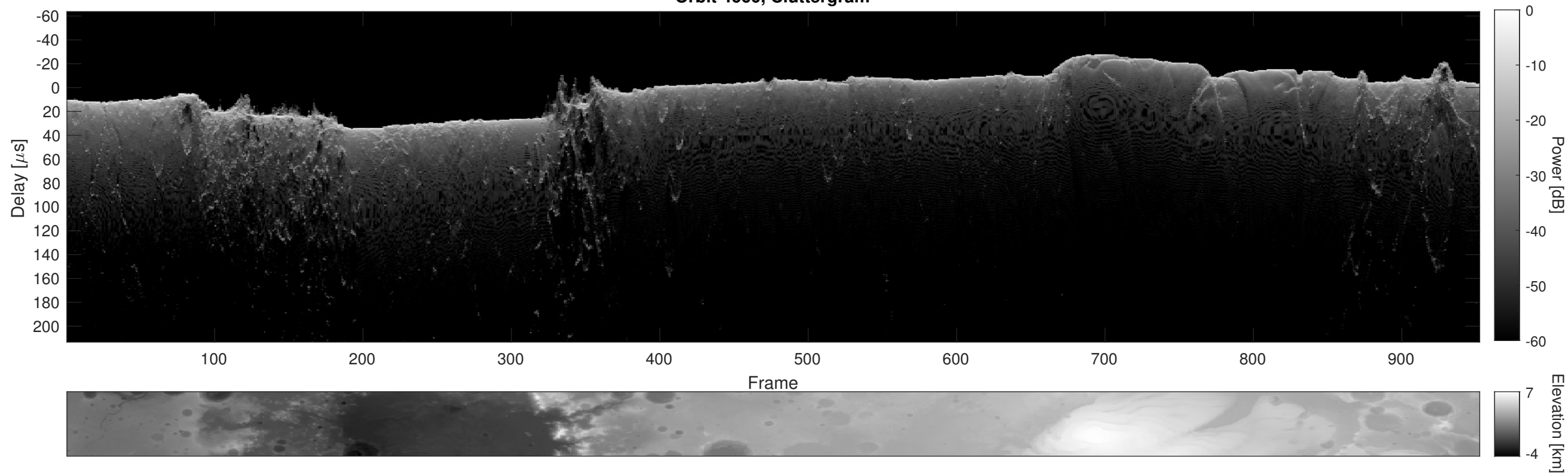
Orbit 4660, Cluttergram
