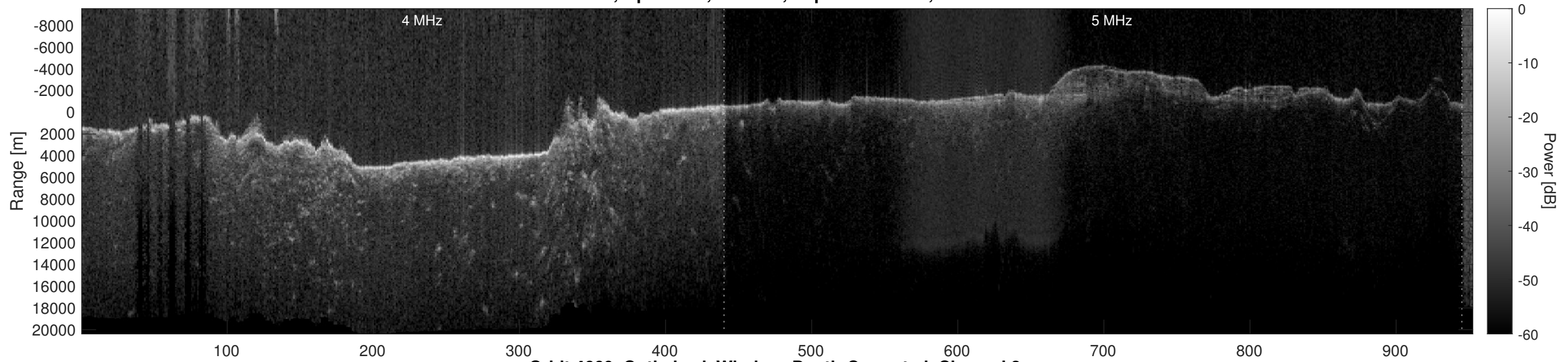
Orbit 4660, Optimized, Window, Depth-Corrected, Channel 2
