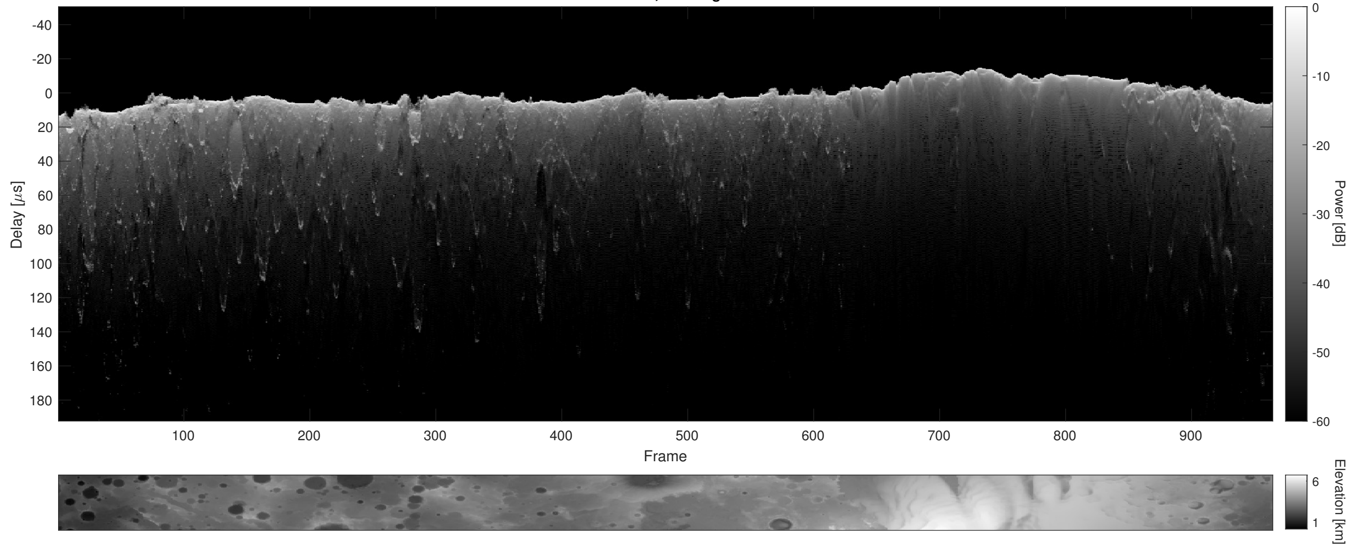
Orbit 4663, Cluttergram
