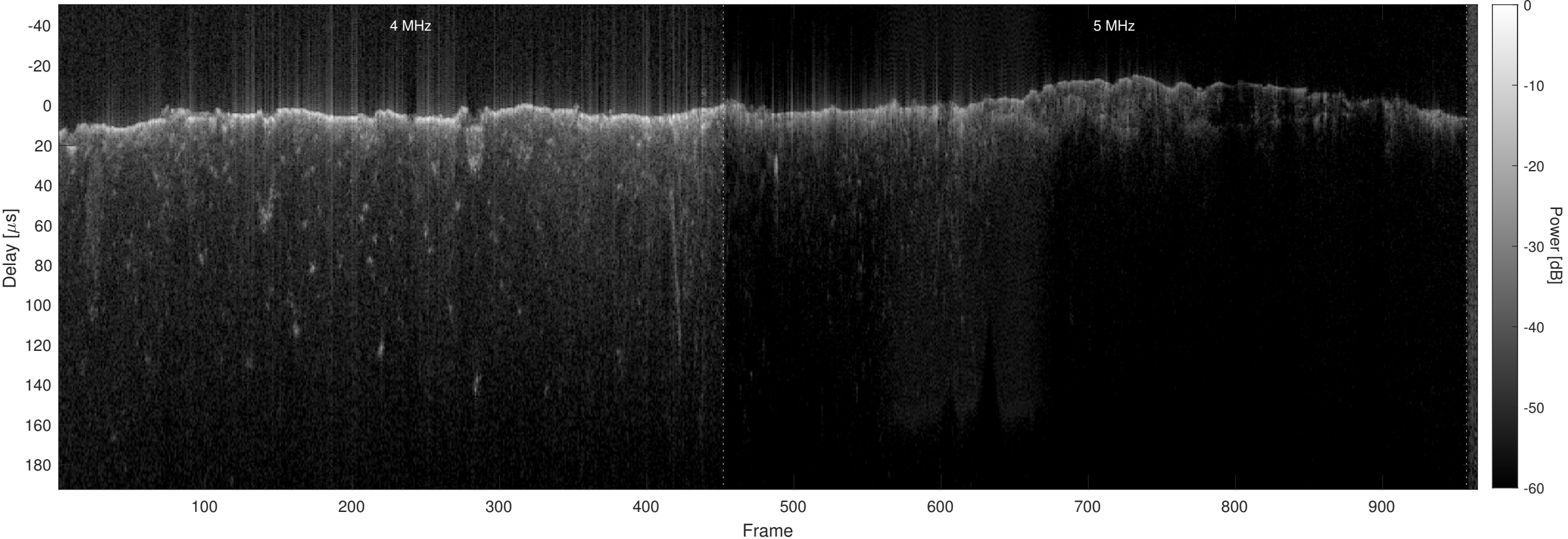
Orbit 4663, Optimized, No Window, Channel 2
