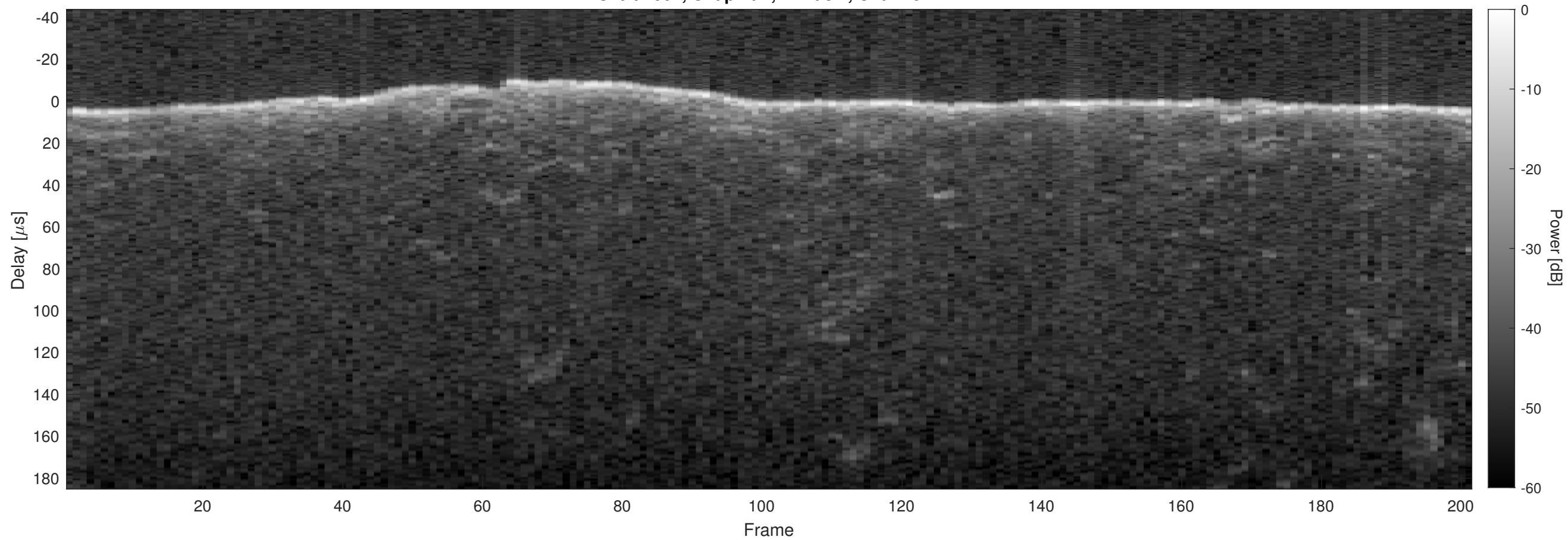
Orbit 4664, Chapman, Window, Channel 2
