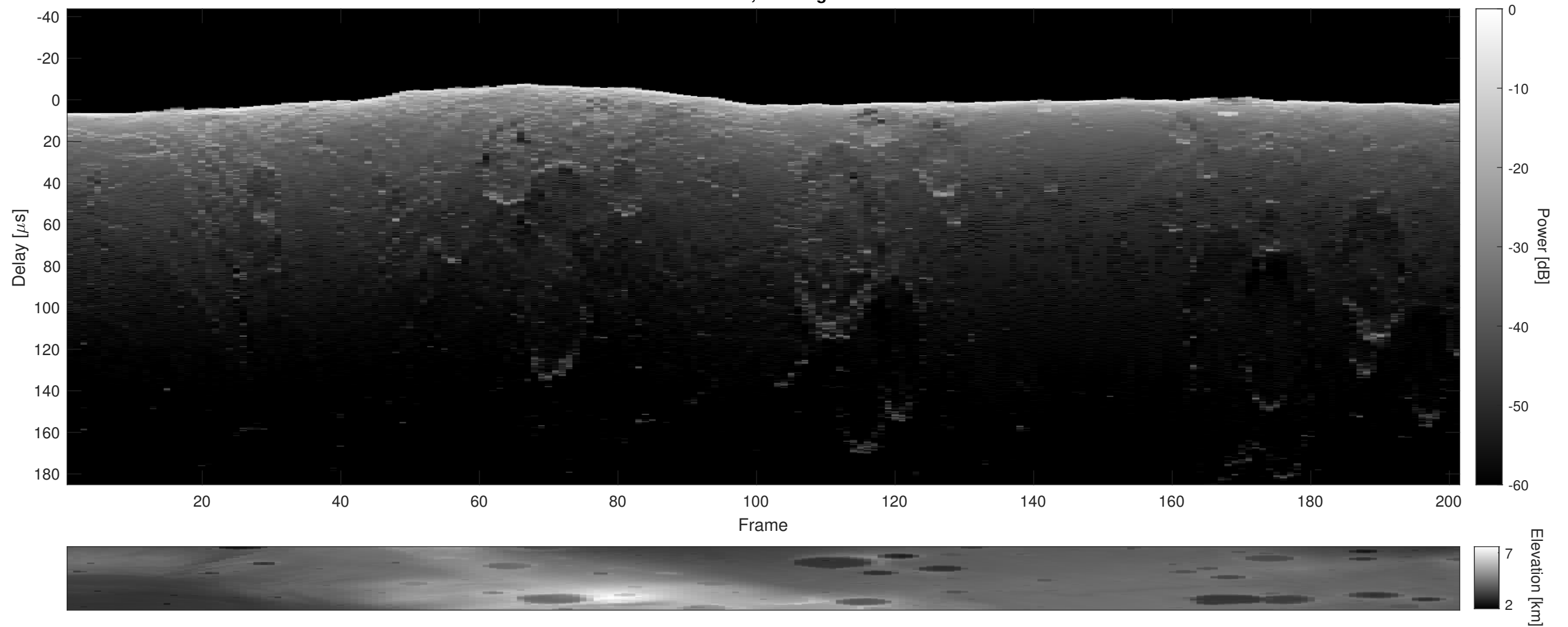
Orbit 4664, Cluttergram
