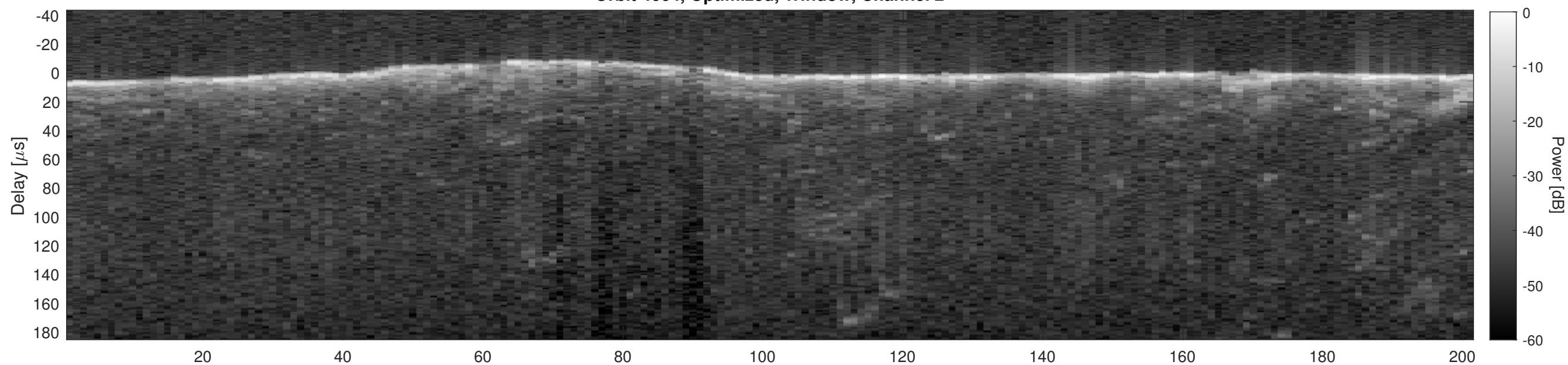
Orbit 4664, Cluttergram
