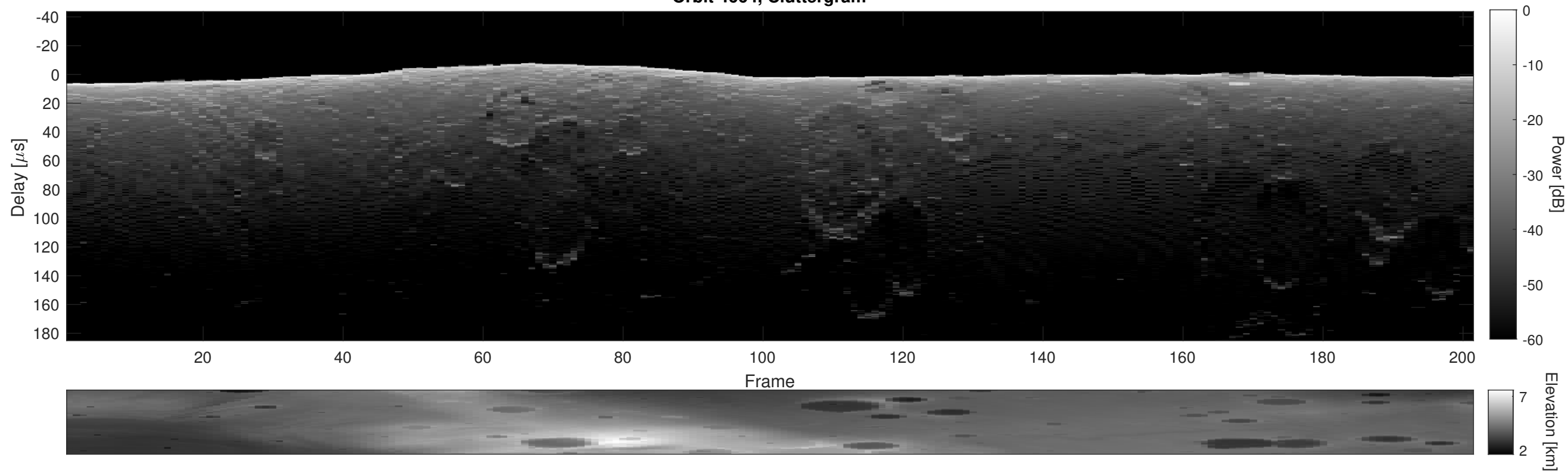
Orbit 4664, Cluttergram
