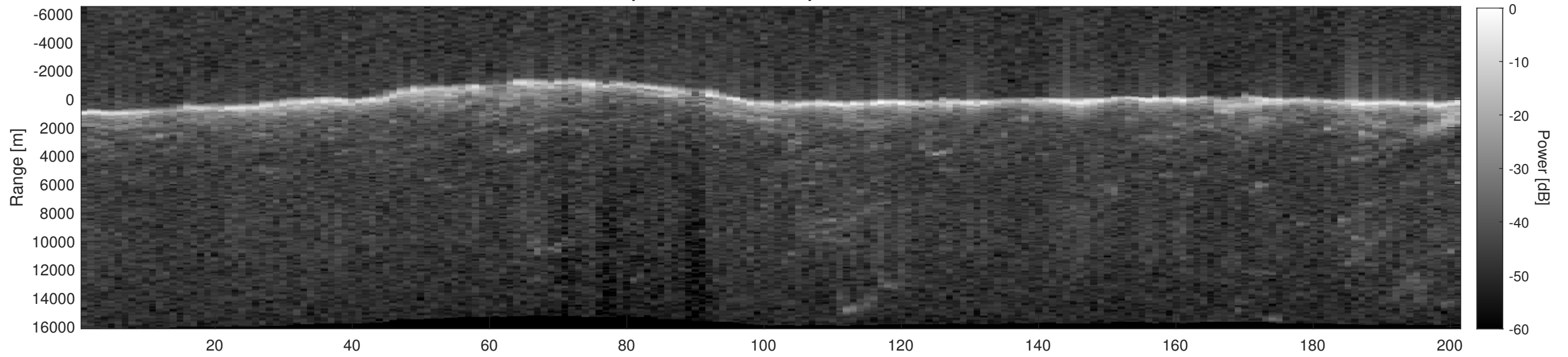
Orbit 4664, Depth-Corrected Cluttergram
