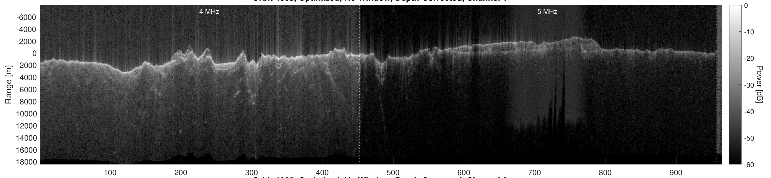
Orbit 4665, Optimized, No Window, Depth-Corrected, Channel 2
