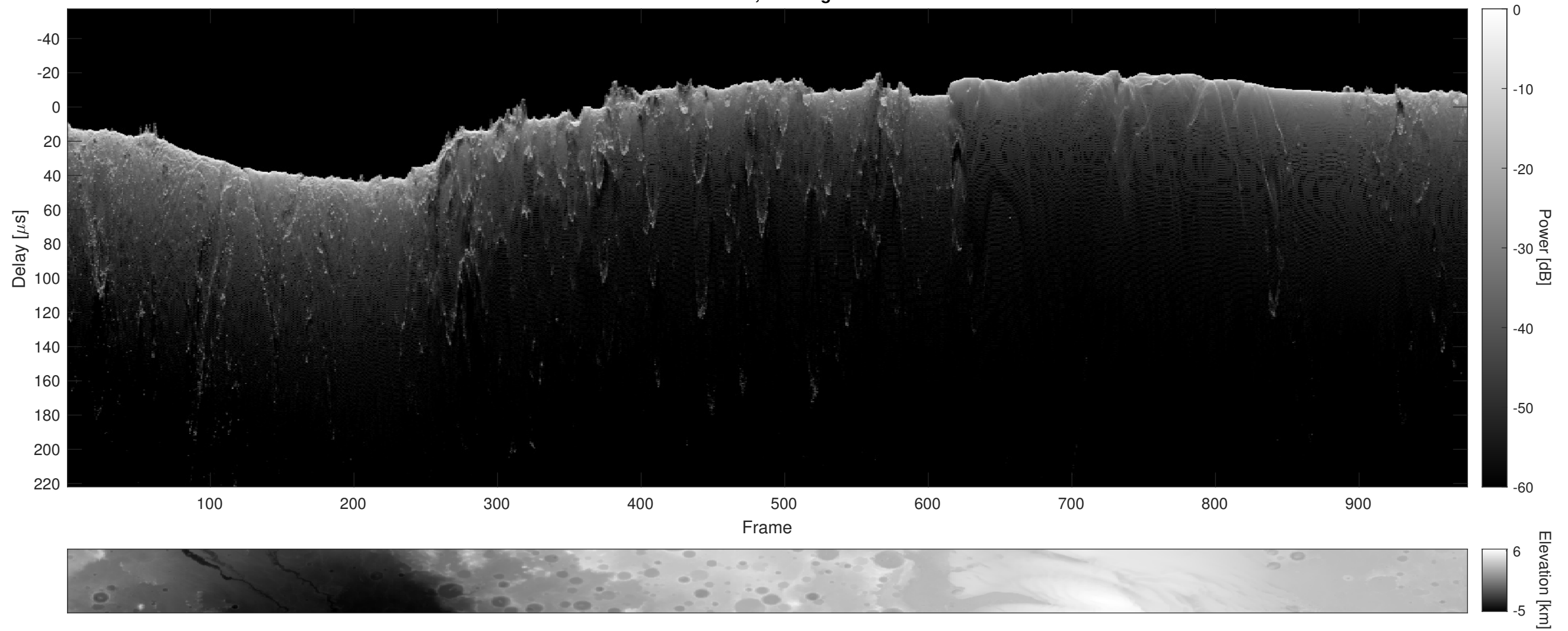
Orbit 4666, Cluttergram
