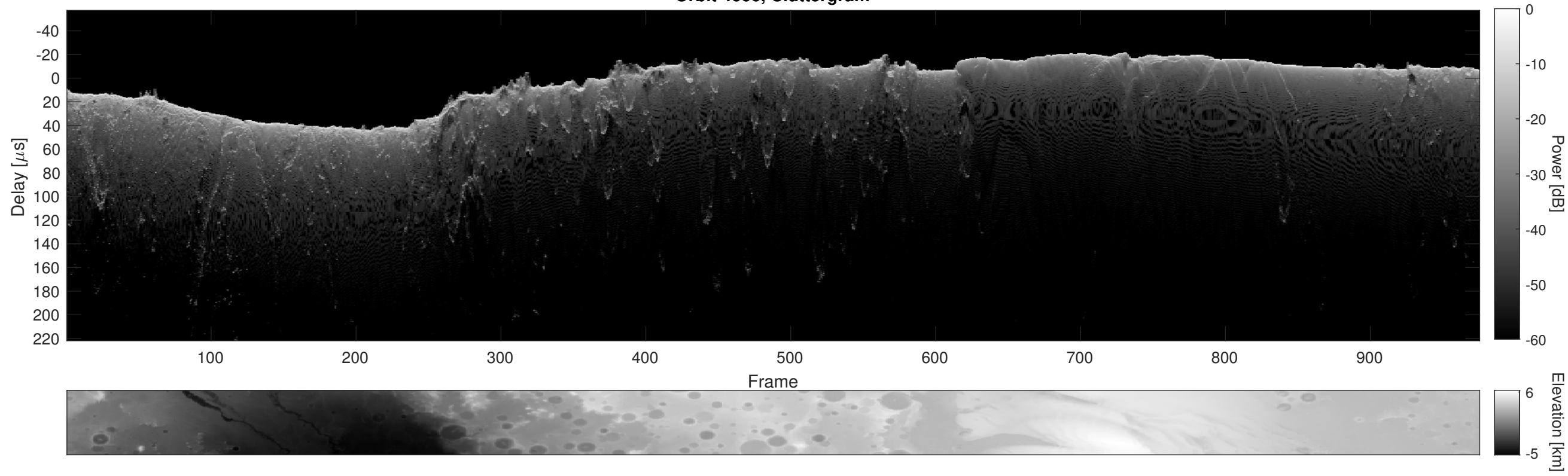
Orbit 4666, Cluttergram
