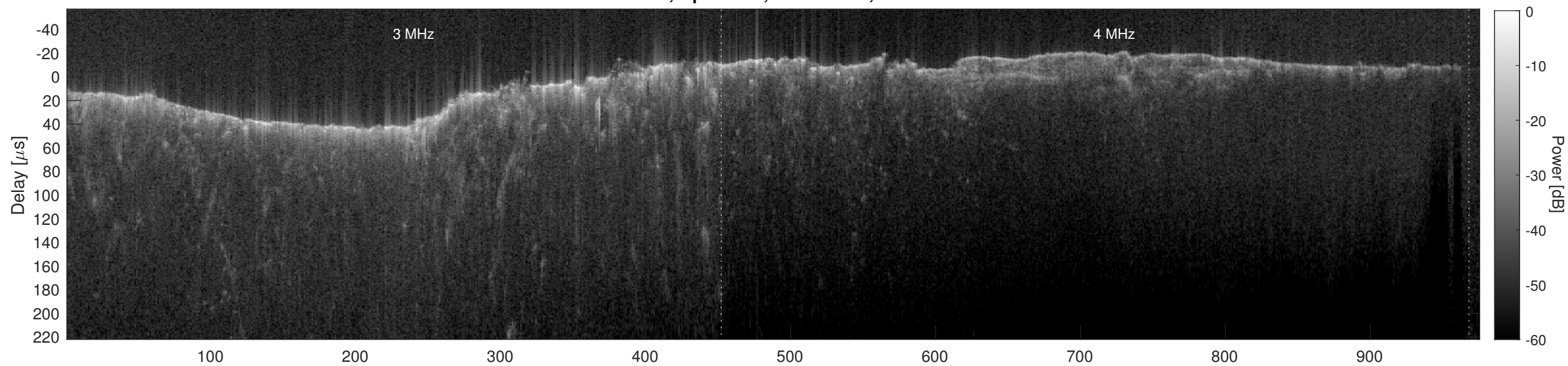
Orbit 4666, Cluttergram
