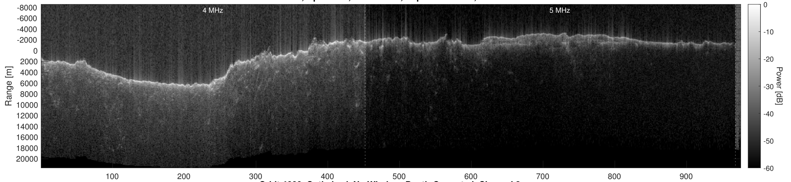
Orbit 4666, Optimized, No Window, Depth-Corrected, Channel 2
