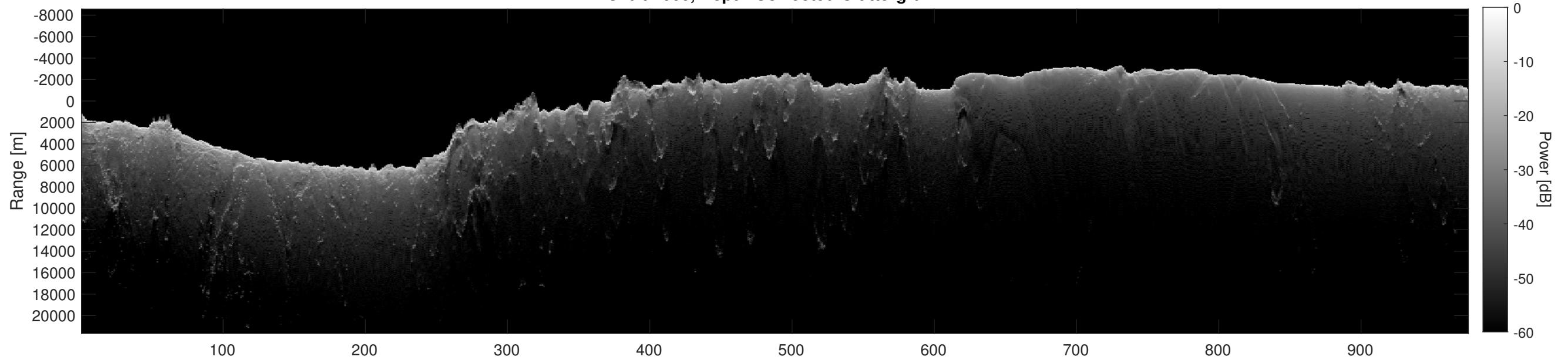
Orbit 4666, Depth-Corrected Cluttergram
