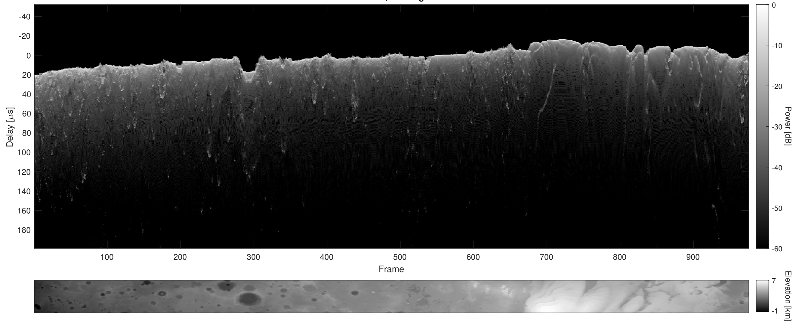
Orbit 4667, Cluttergram
