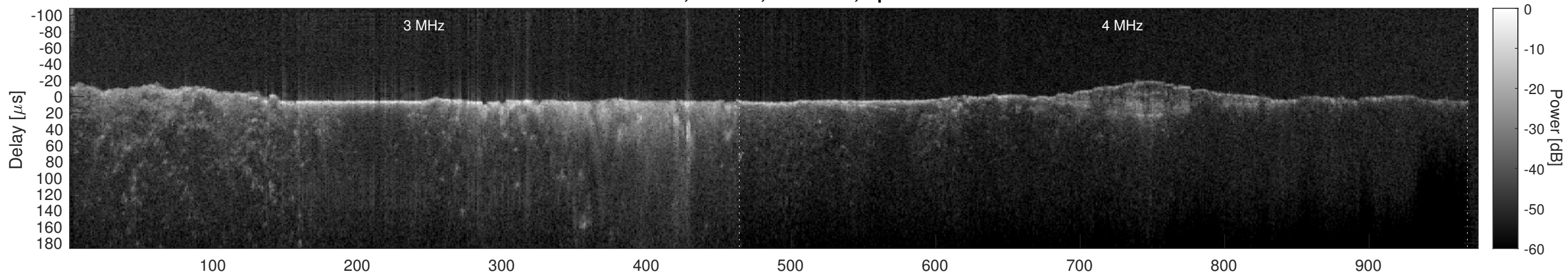
Orbit 4668, Cluttergram
