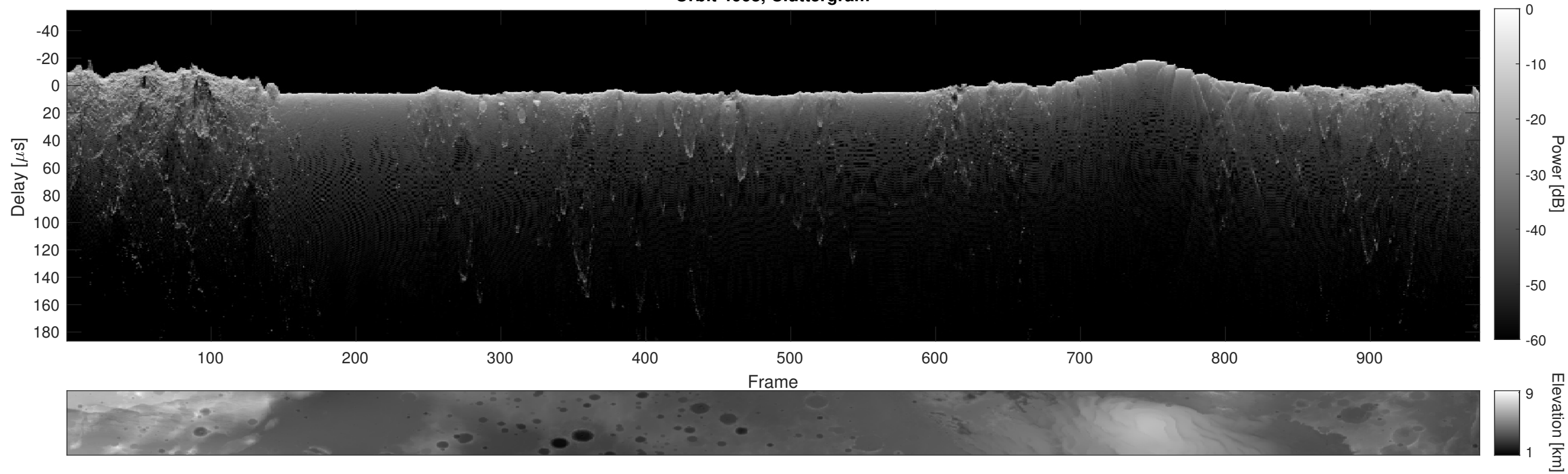
Orbit 4668, Cluttergram
