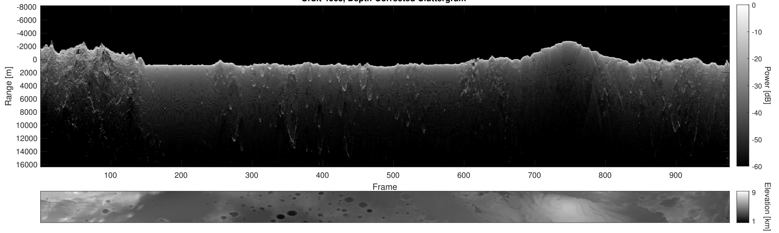
Orbit 4668, Depth-Corrected Cluttergram
