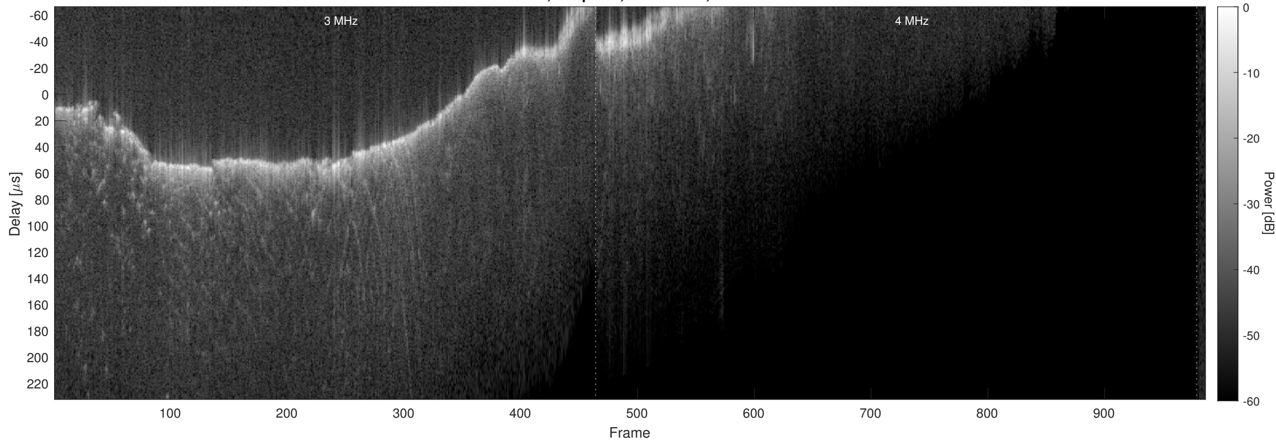
Orbit 4670, Chapman, No Window, Channel 2
