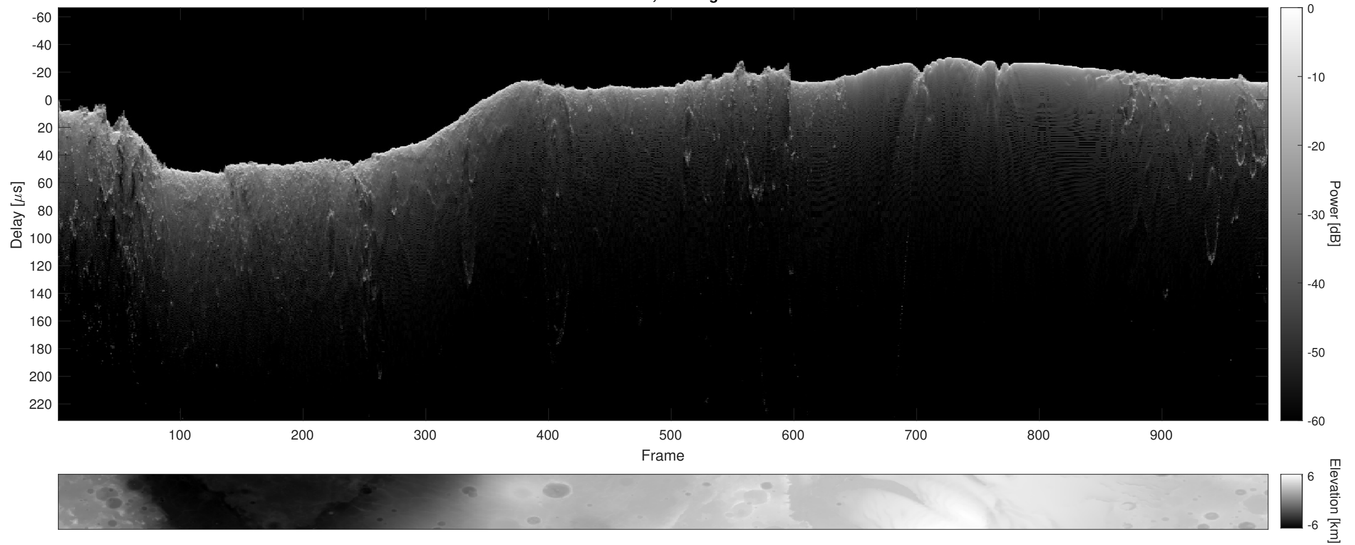
Orbit 4670, Cluttergram
