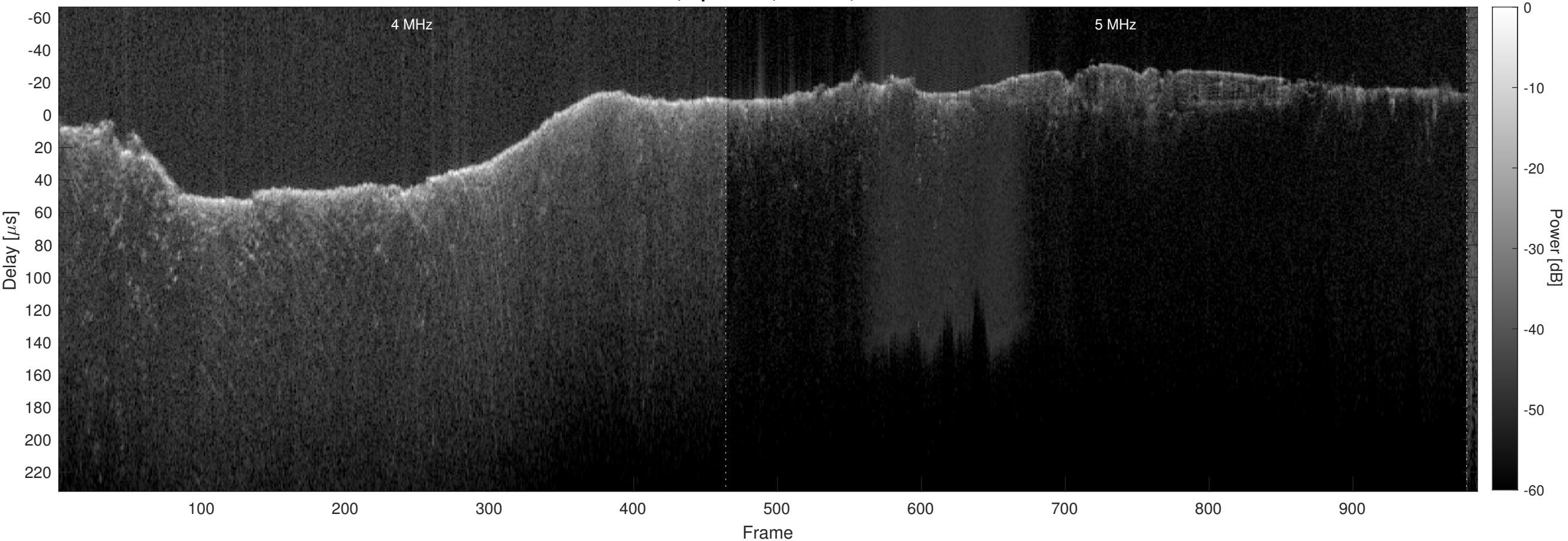
Orbit 4670, Optimized, Window, Channel 2
